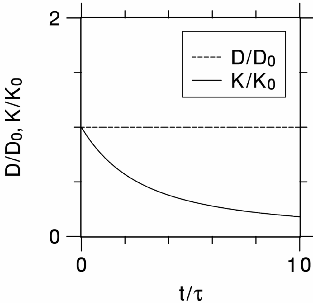
Figure 1. Time dependence of the diffusion coefficient and diffusional kurtosis for the Kärger model. The diffusion coefficient is independent of the diffusion time, but the kurtosis decreases on a time scale set by the water exchange time \tau .
